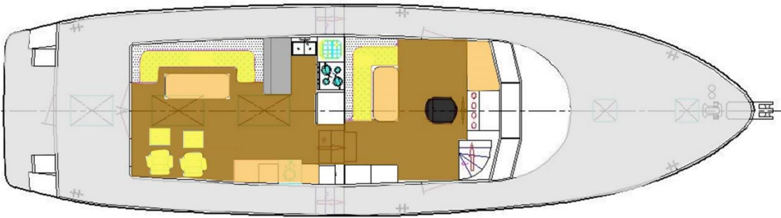
Layout: Main Deck – Saloon, Galley, and Raised Pilothouse
