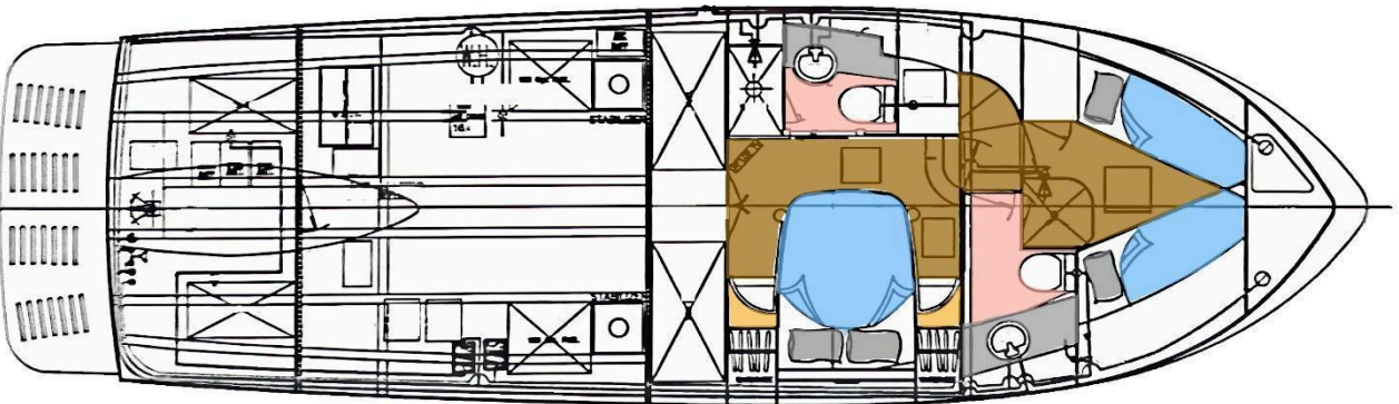
LAYOUT: Lower Deck – Engine Room, Staterooms, Heads
